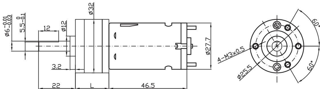
DRAWING (MM)
