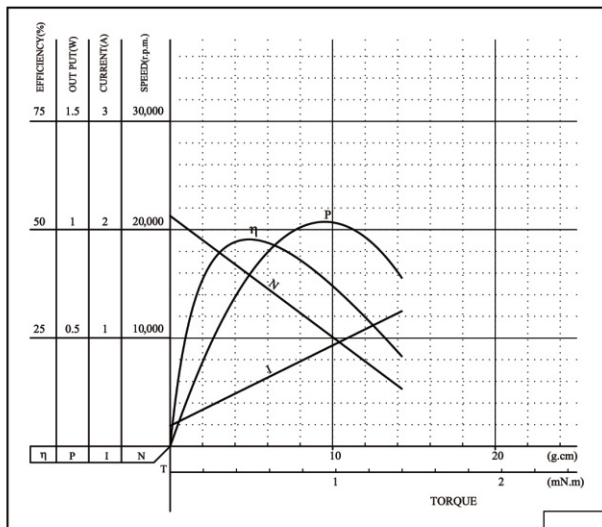
MODEL: DSD-1220CA-1396
