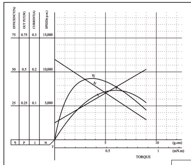
MODEL: DSD-1220CA-1585
