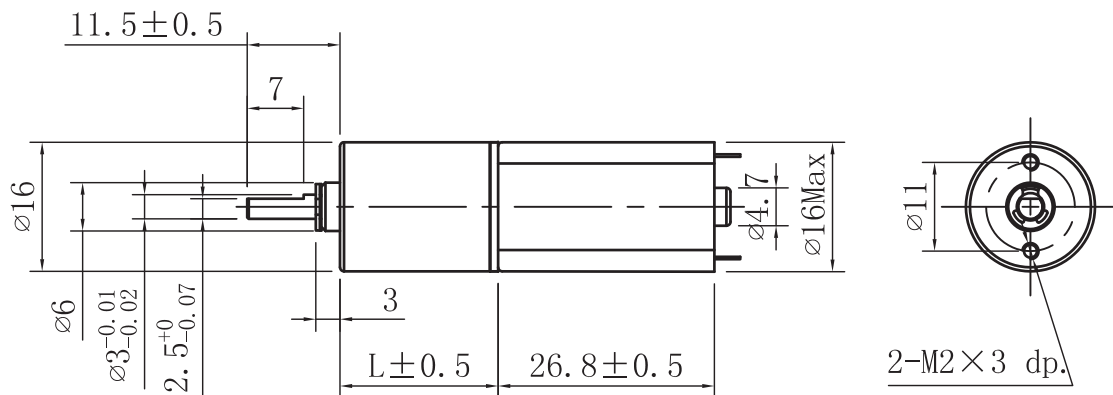
DRAWING (MM)
