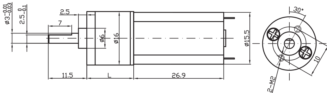
DRAWING (MM)
