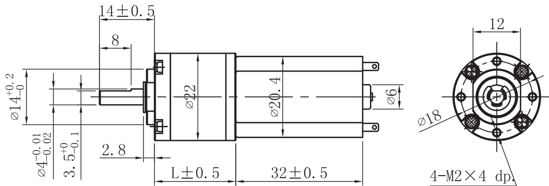
DRAWING (MM)
