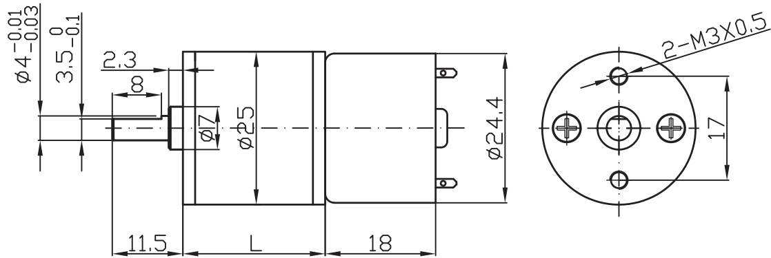
DRAWING (MM)
