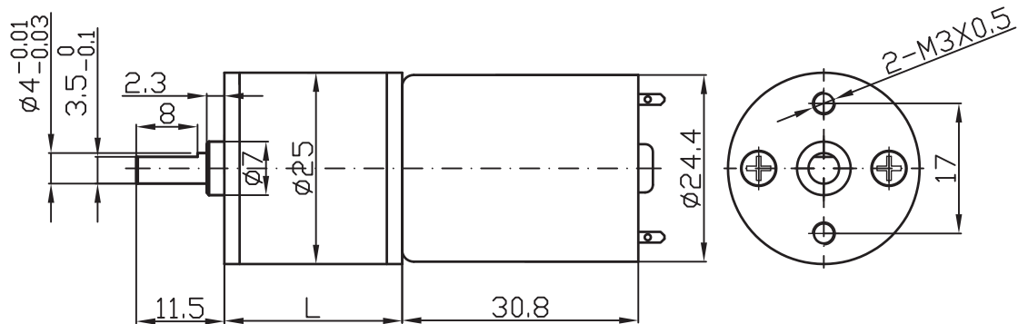
DRAWING (MM)
