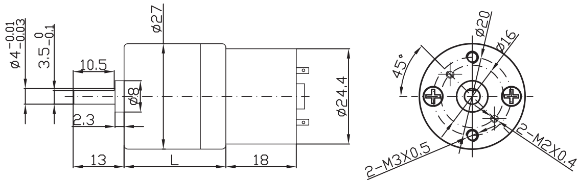
DRAWING (MM)
