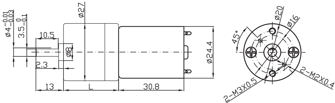
DRAWING (MM)
