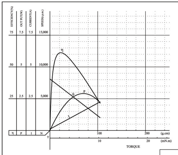
MODEL: DSD-280SA-2290
