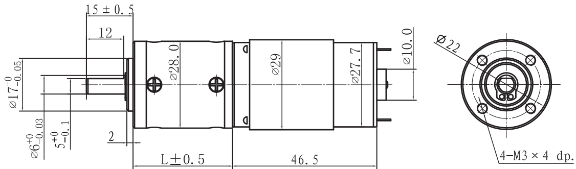
DRAWING (MM)
