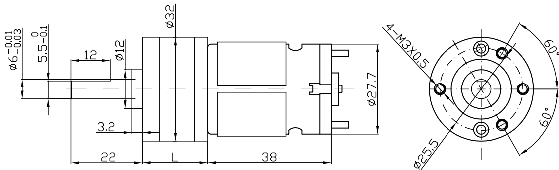
DRAWING (MM)
