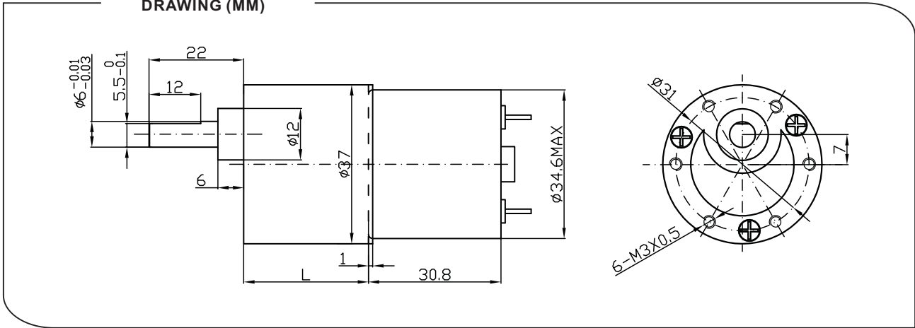
DRAWING (MM)
