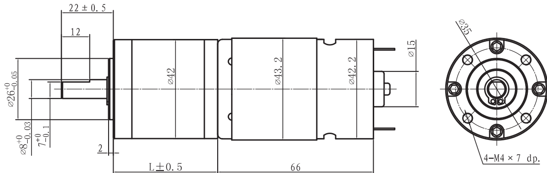
DRAWING (MM)
