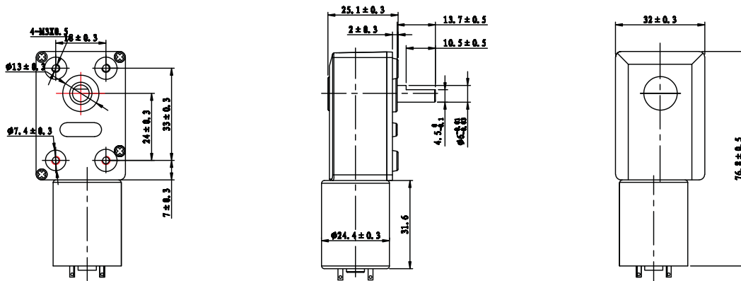
DRAWING (MM)
