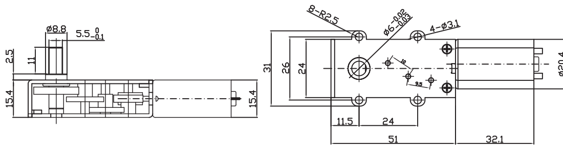
DRAWING (MM)
