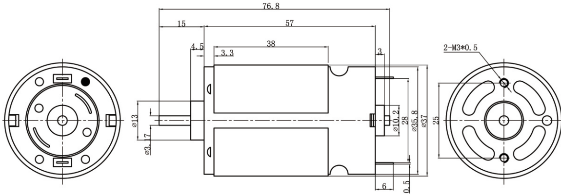
DRAWING (MM)
