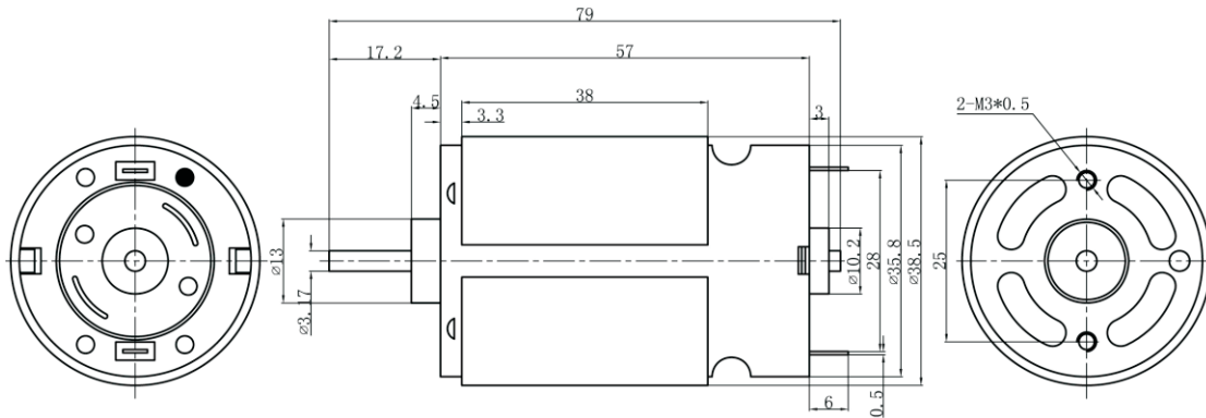
DRAWING (MM)
