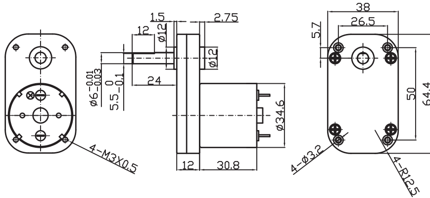
DRAWING (MM)
