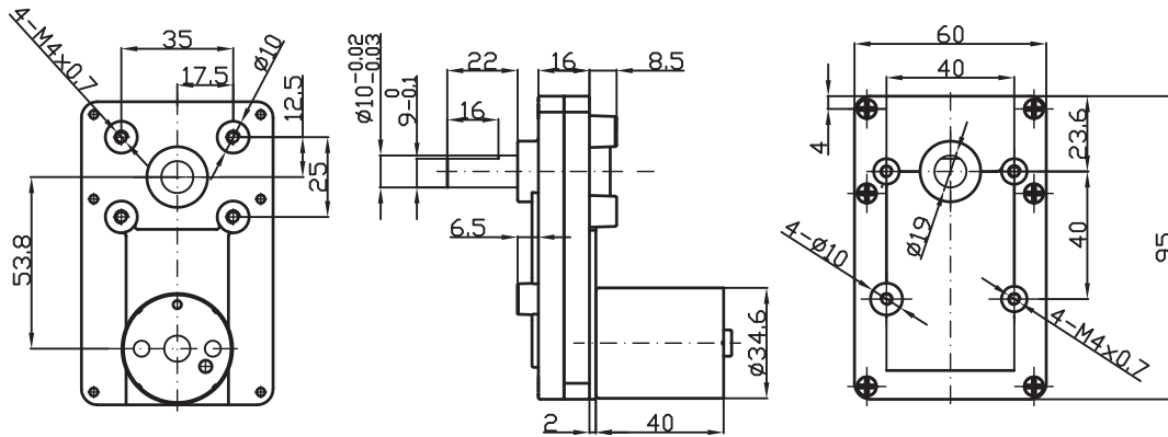
DRAWING (MM)
