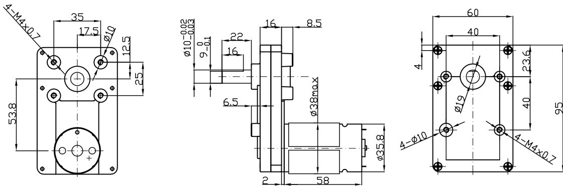
DRAWING (MM)
